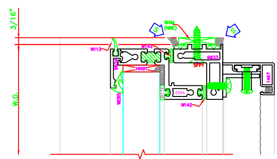
102 HEAD WV410
