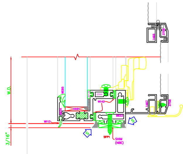
202 SILL WV410
